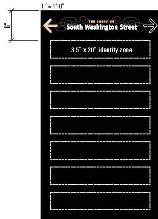
24 x 42 insert Single digital print applied to substrate (7) listings module Qty (2) panels per A-frame Recommend BLACK background Panel thickness min. 1/8", max. 1/4"
