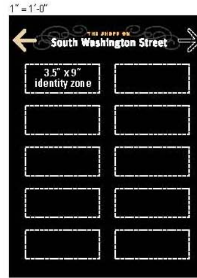
24 x 32 insert Single digital print applied to substrate (10) listings module Qty (2) panels per A-frame Recommend BLACK background Panel thickness min. 1/8", max. 1/4"
